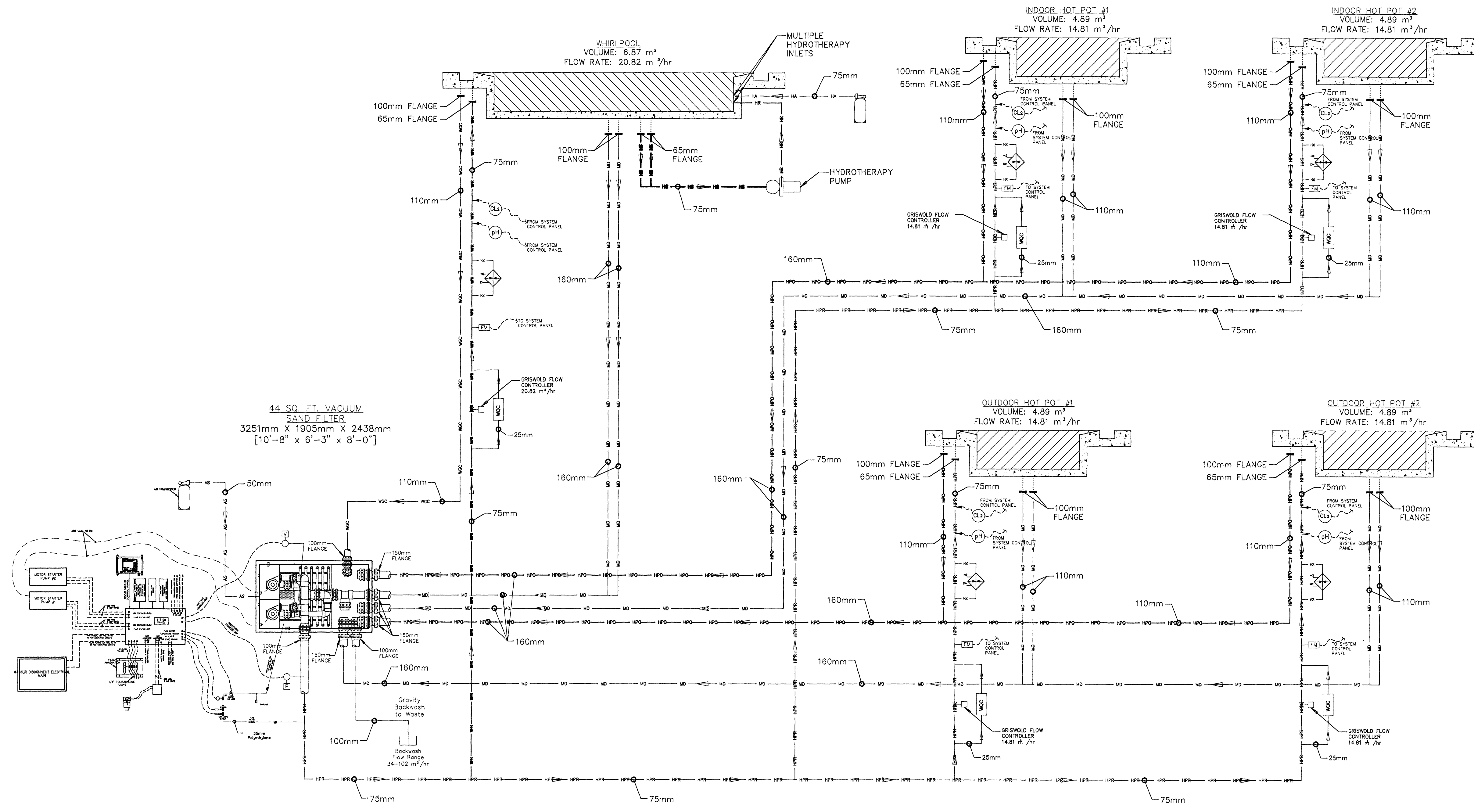
WHIRLPOOL - HOT POTS HYDRAULIC FLOW SCHEMATIC
