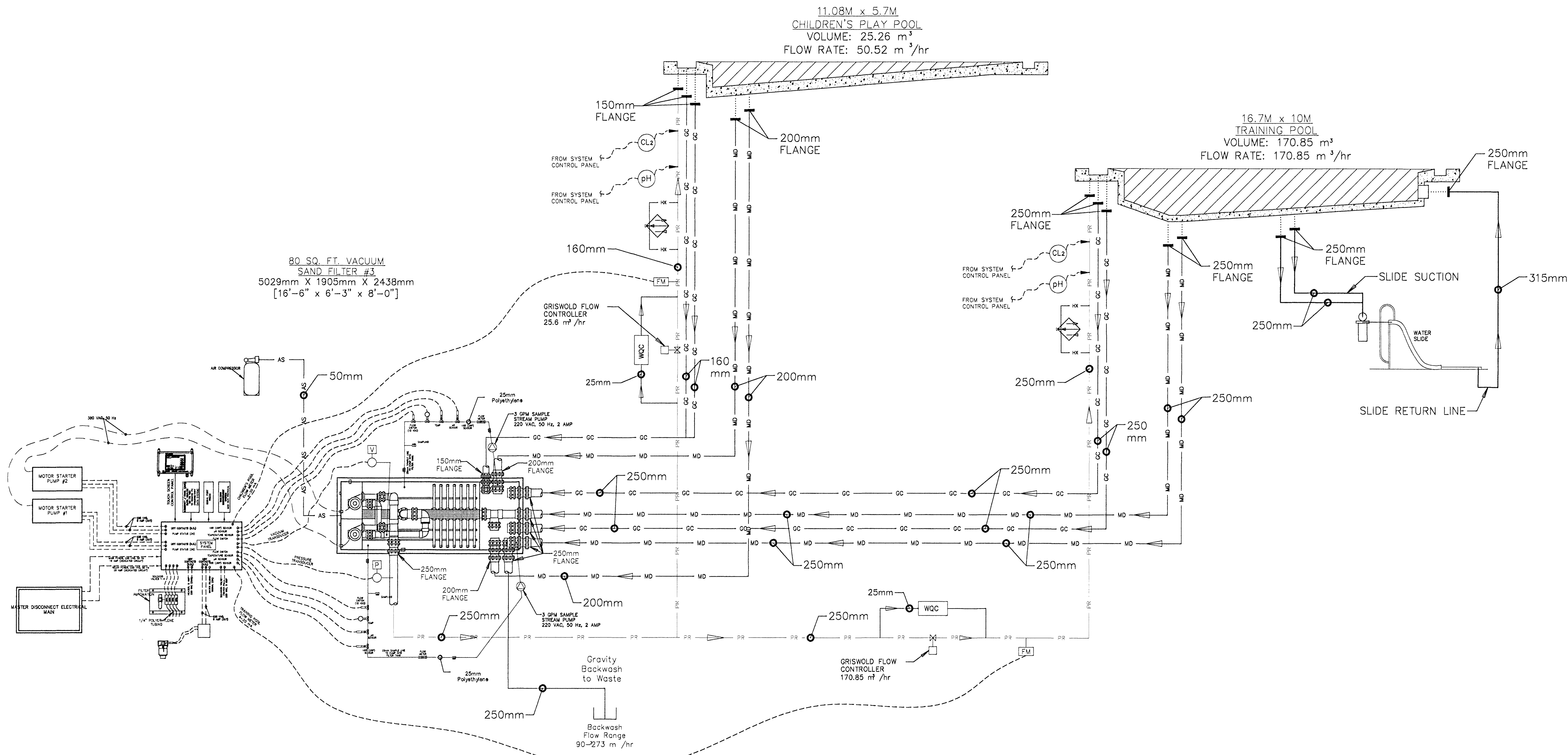
CHILDREN'S POOL - TRAINING POOL HYDRAULIC FLOW SCHEMATIC
