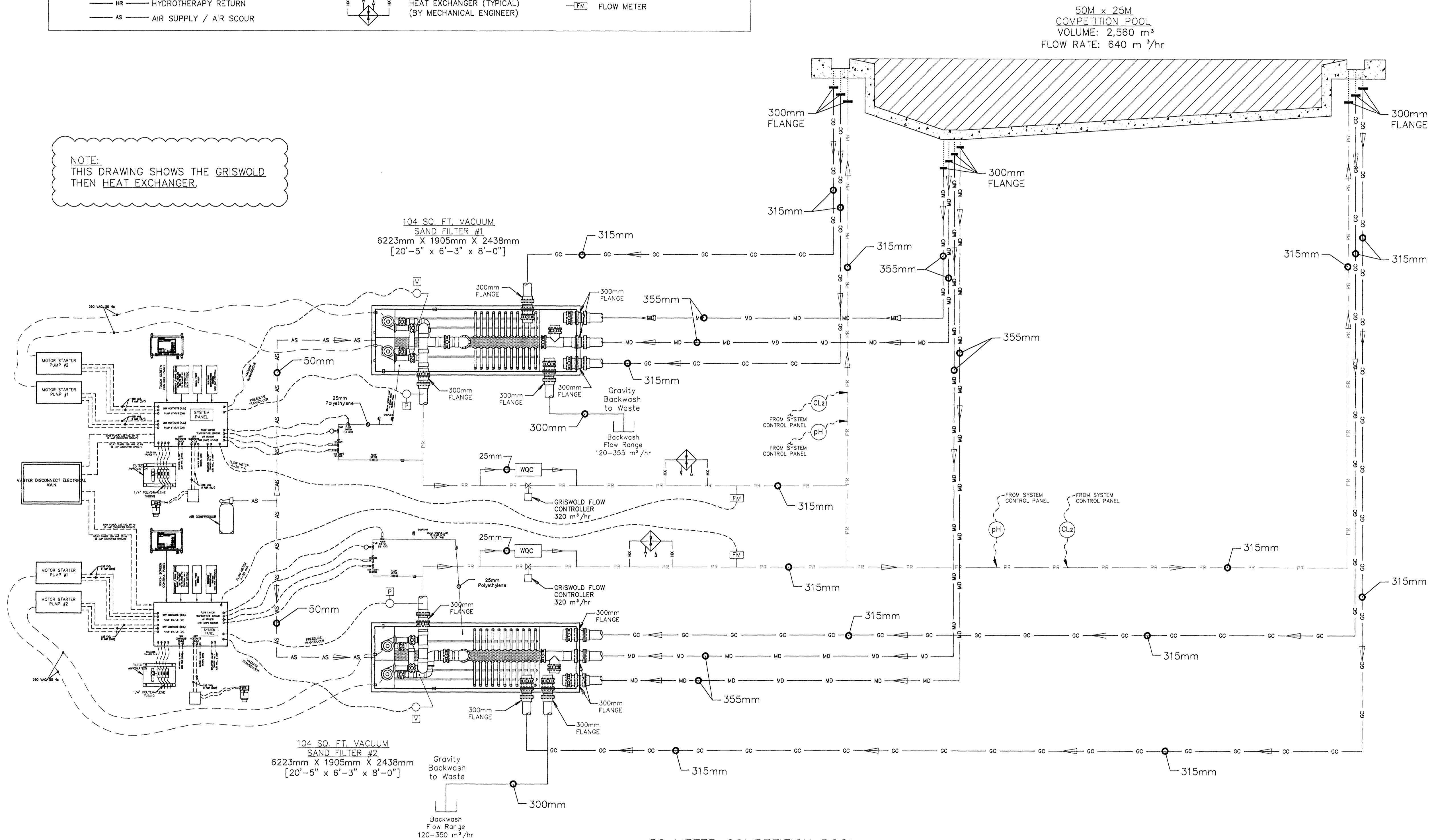
50 METER COMPETITION POOL HYDRAULIC FLOW SCHEMATIC GRISWOLD THEN HEAT EXCHANGER
