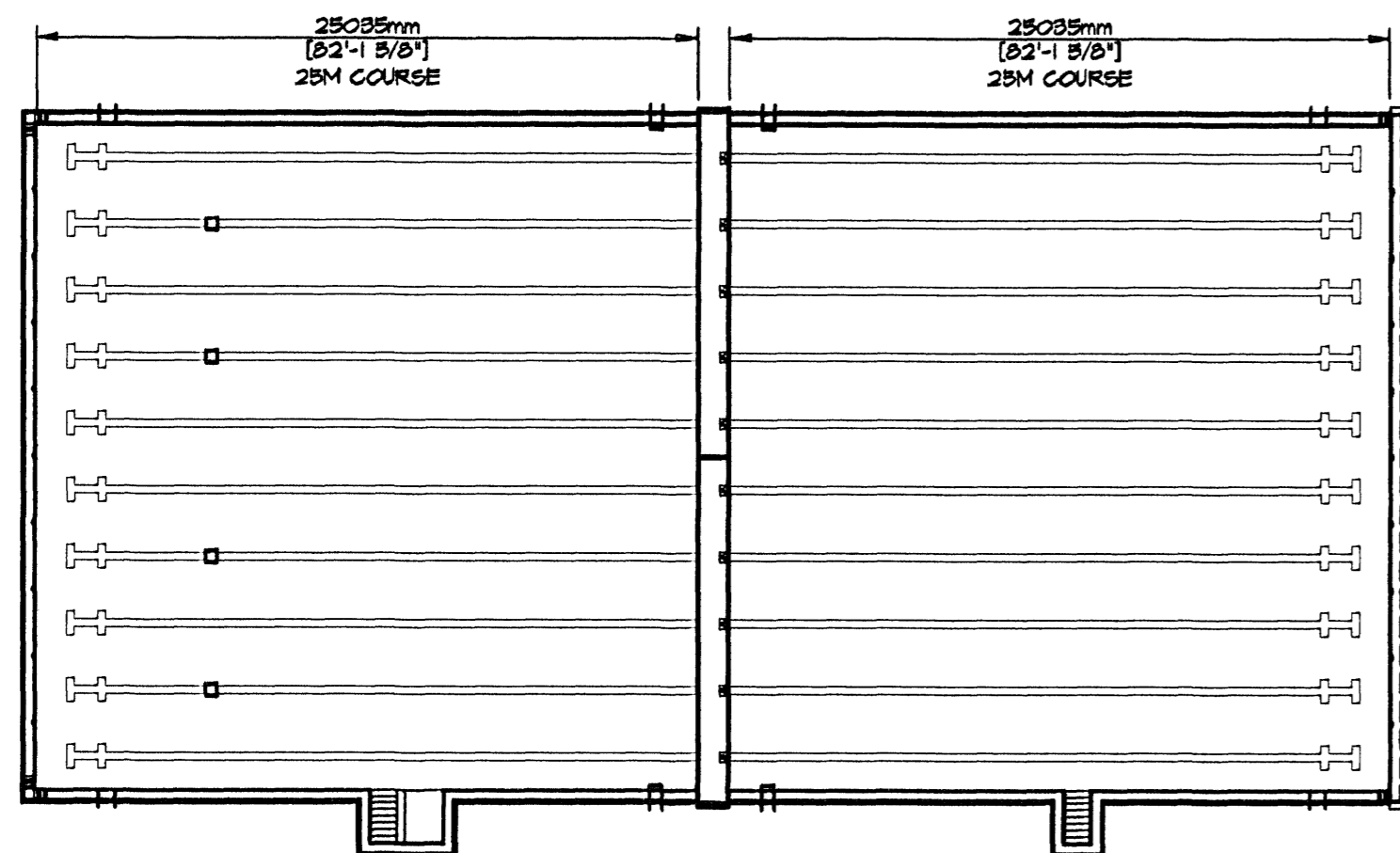
B 7.4 BULKHEAD LOCATION PLAN
