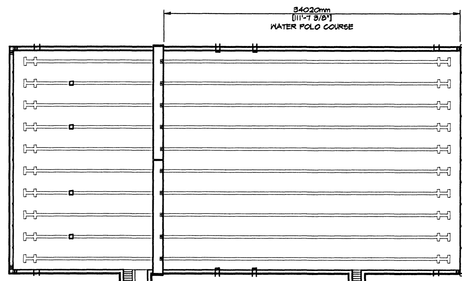
E 7.4 BULKHEAD LOCATION PLAN
