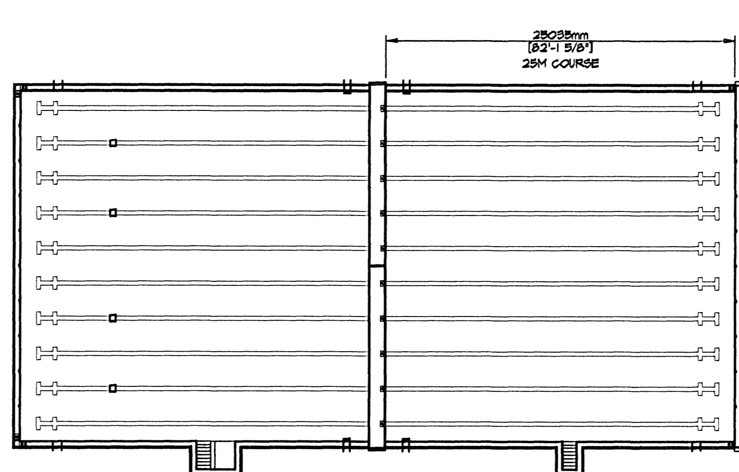
F 7.4 BULKHEAD LOCATION PLAN
