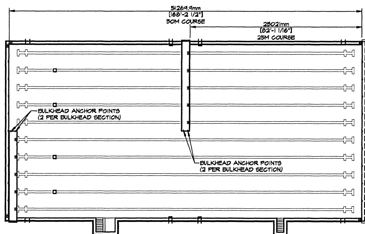
C 7.4 BULKHEAD LOCATION PLAN
