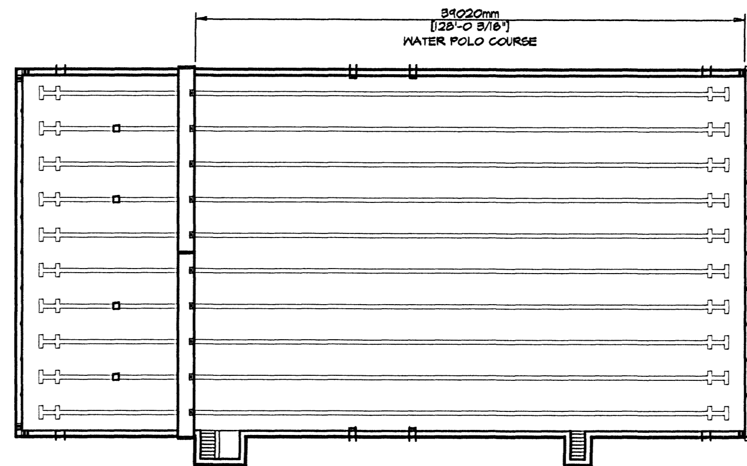
D 7.4 BULKHEAD LOCATION PLAN
