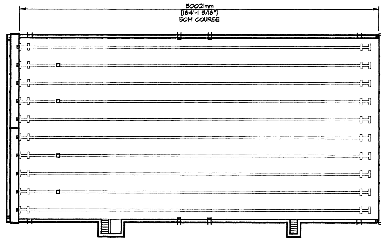
A 7.4 BULKHEAD LOCATION PLAN
