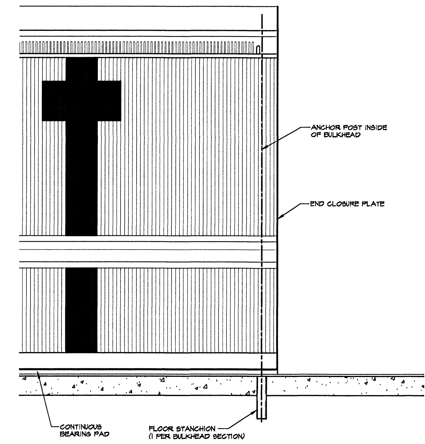
(B) ELEVATION ANCHOR DETAIL
