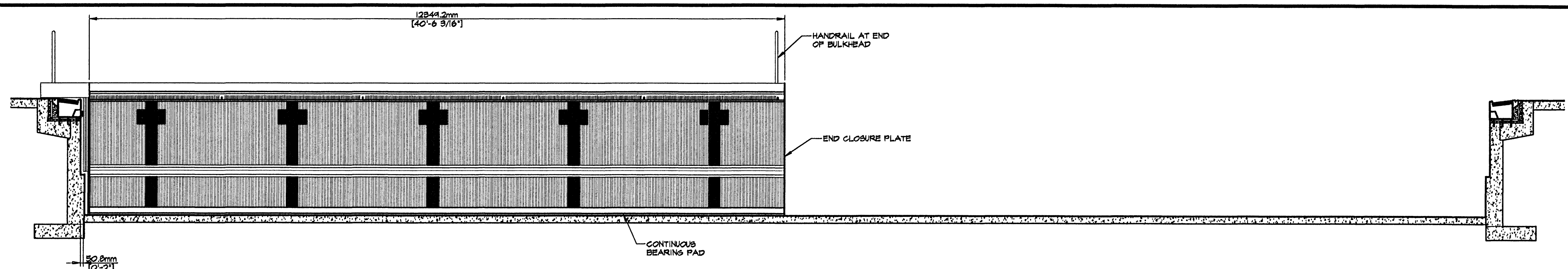
(A) SPLIT BULKHEAD DETAIL
