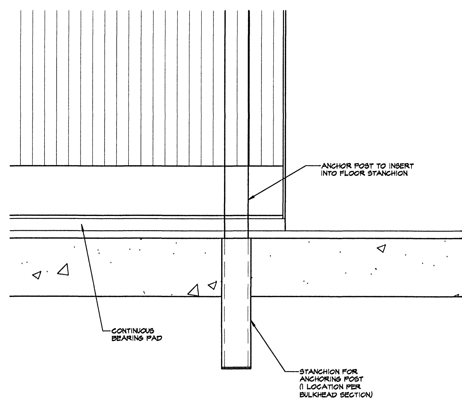
(C) FLOOR ANCHORING DETAIL
