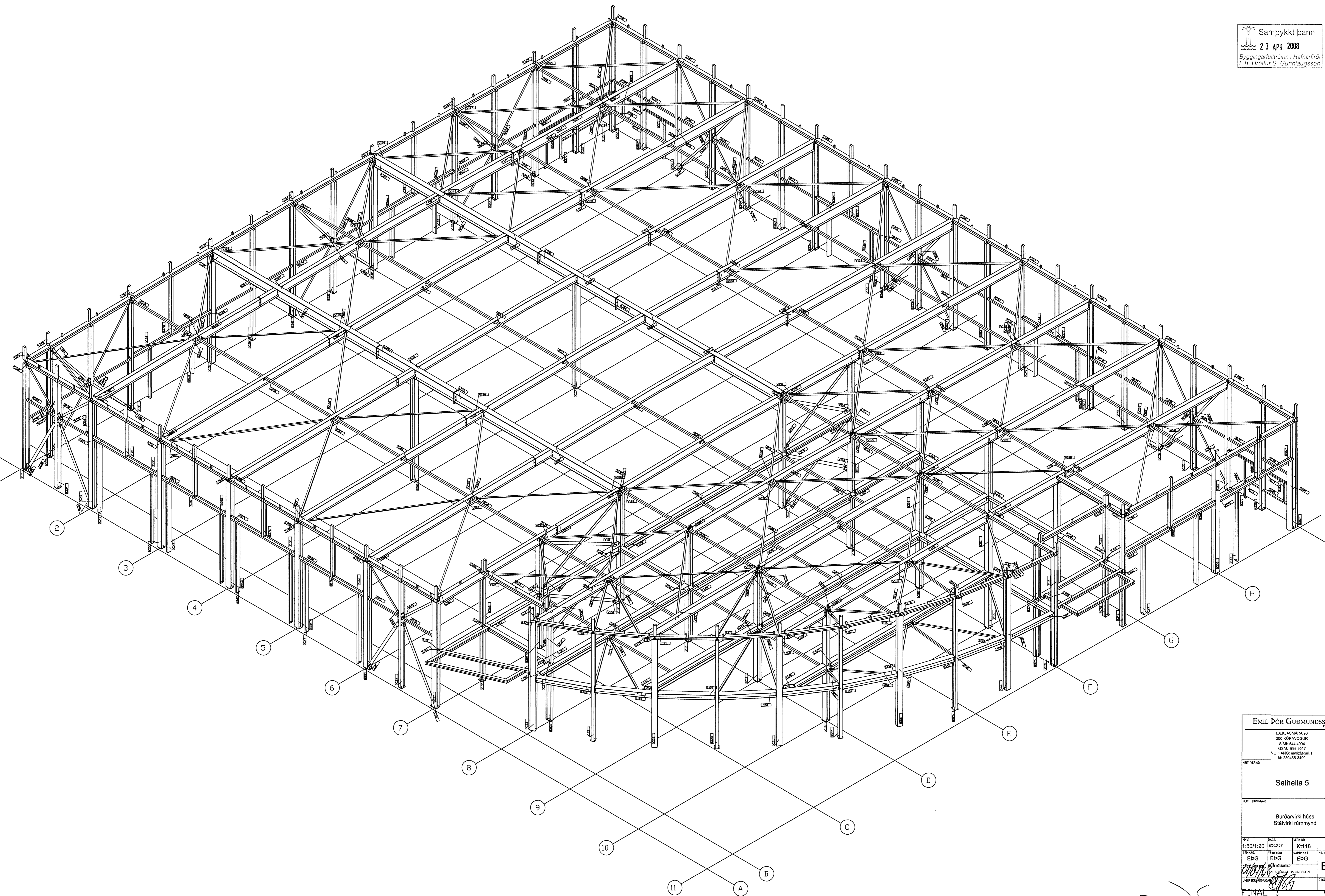
3-D View
