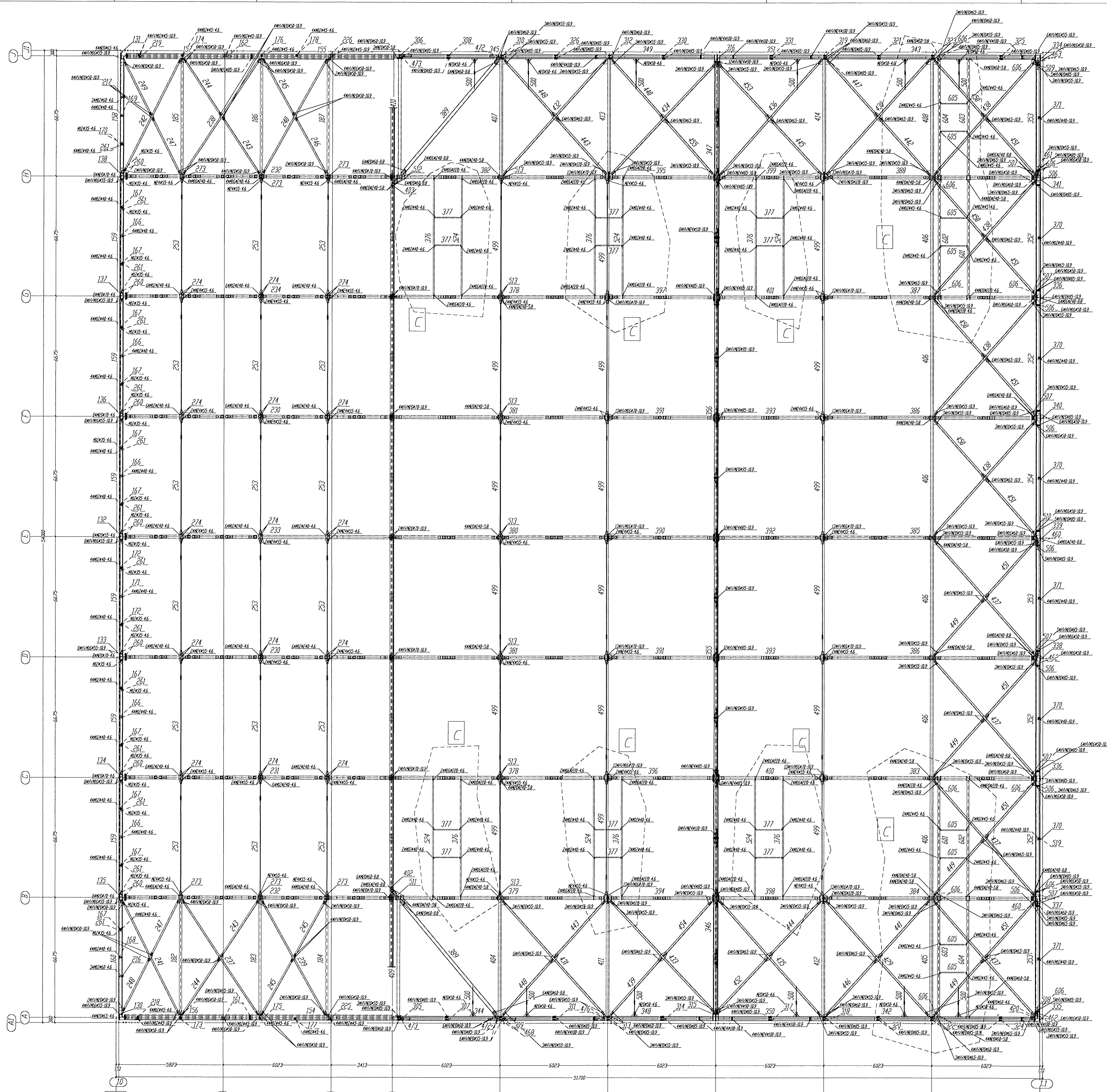
ROOF Sc. 1:75
