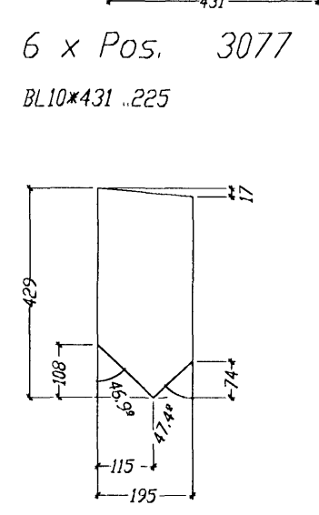
6 x Pos. 3077 BL10*431.225
