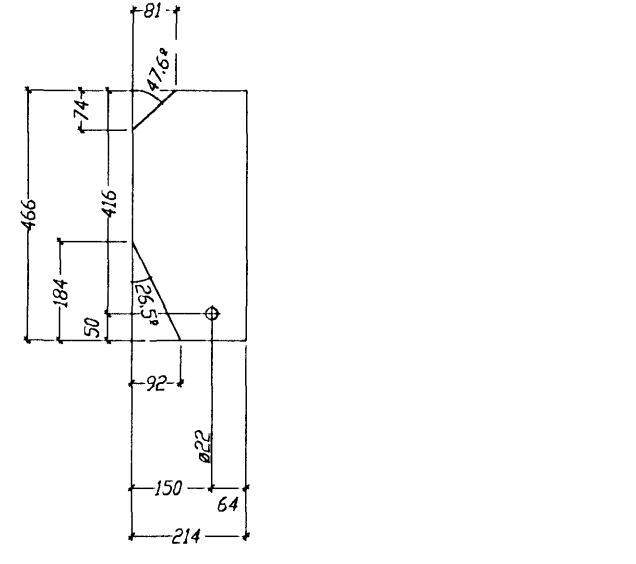
4 x Pos. 3070 BL10*466.214
