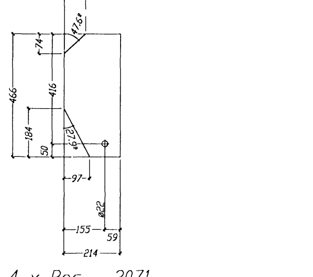
4 x Pos. 3071 BL10*466.214
