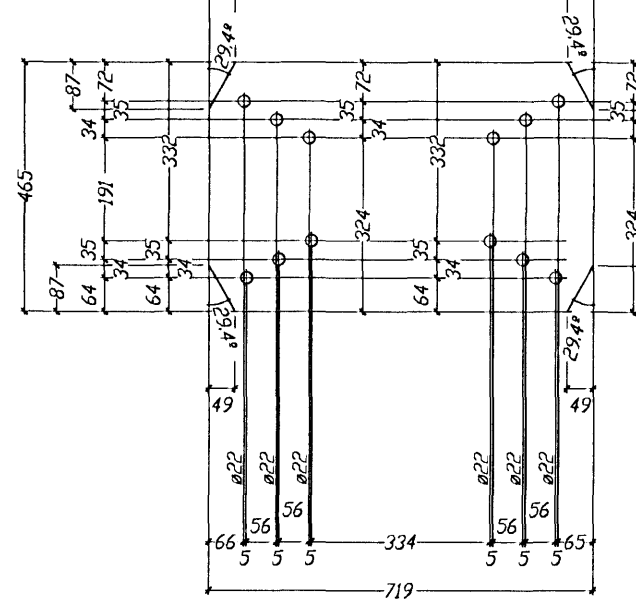
3 x Pos. 3072 BL10*465 - S235J2G3.719
