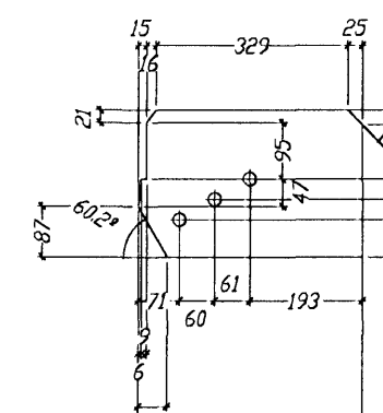
3 x Pos. 3092 BL10*385.250
