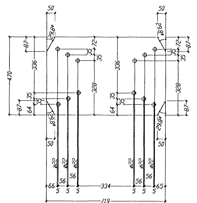
3 x Pos. 3069 BL10*470 - S235J2G3.719
