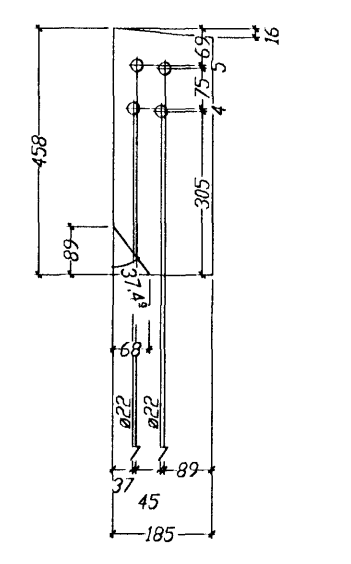
5 x Pos. 3074 BL12*458 - S235J2G3.185
