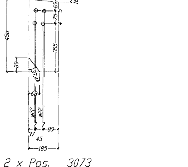
2 x Pos. 3073 BL12*458 - S235J2G3.185
