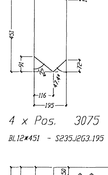
4 x Pos. 3075 BL12*451 - S235J2G3.195
