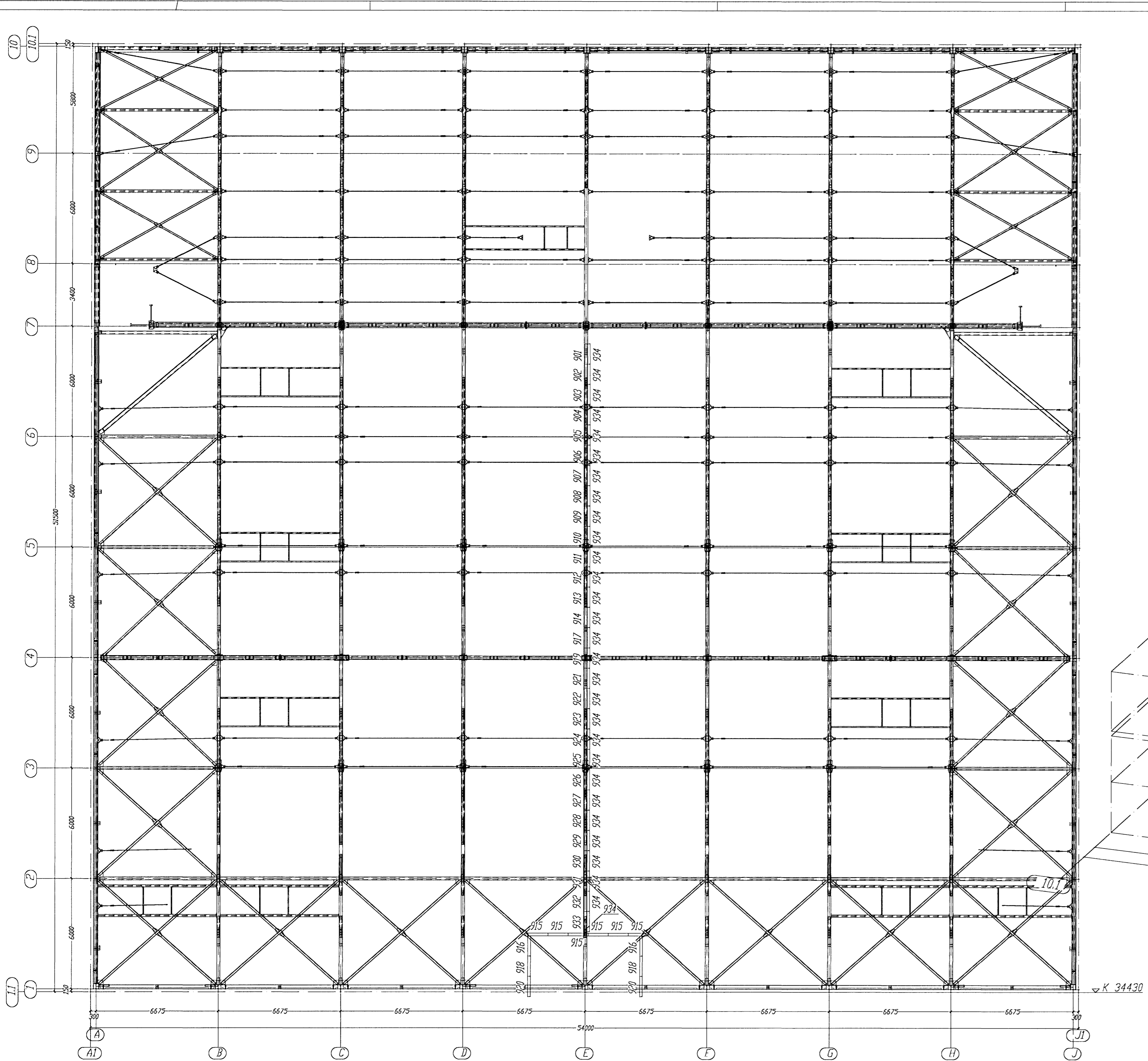
ROOF Sc. 1:100
