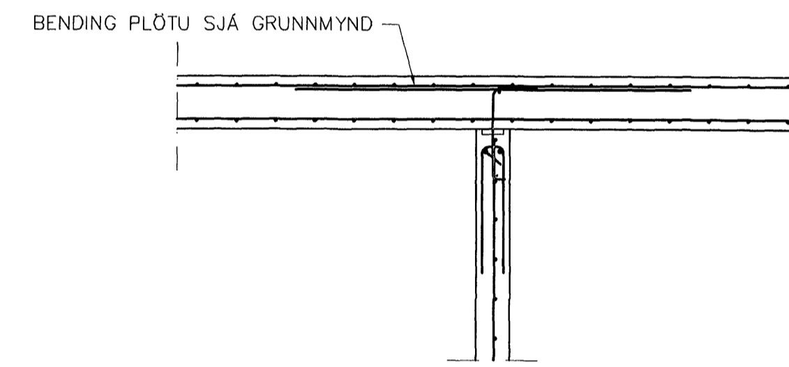
SNID 2-2 1:20
