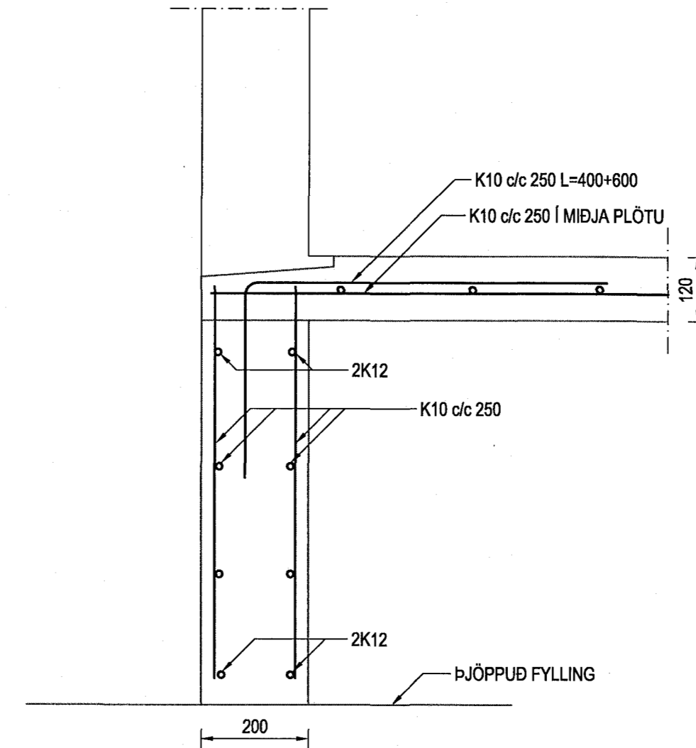
SNID 4-4 MKV. 1:10
