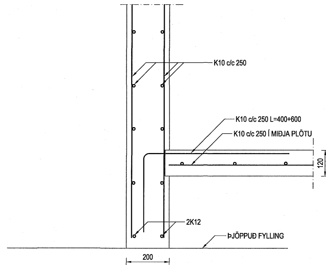
SNID 2-2 MKV. 1:10
