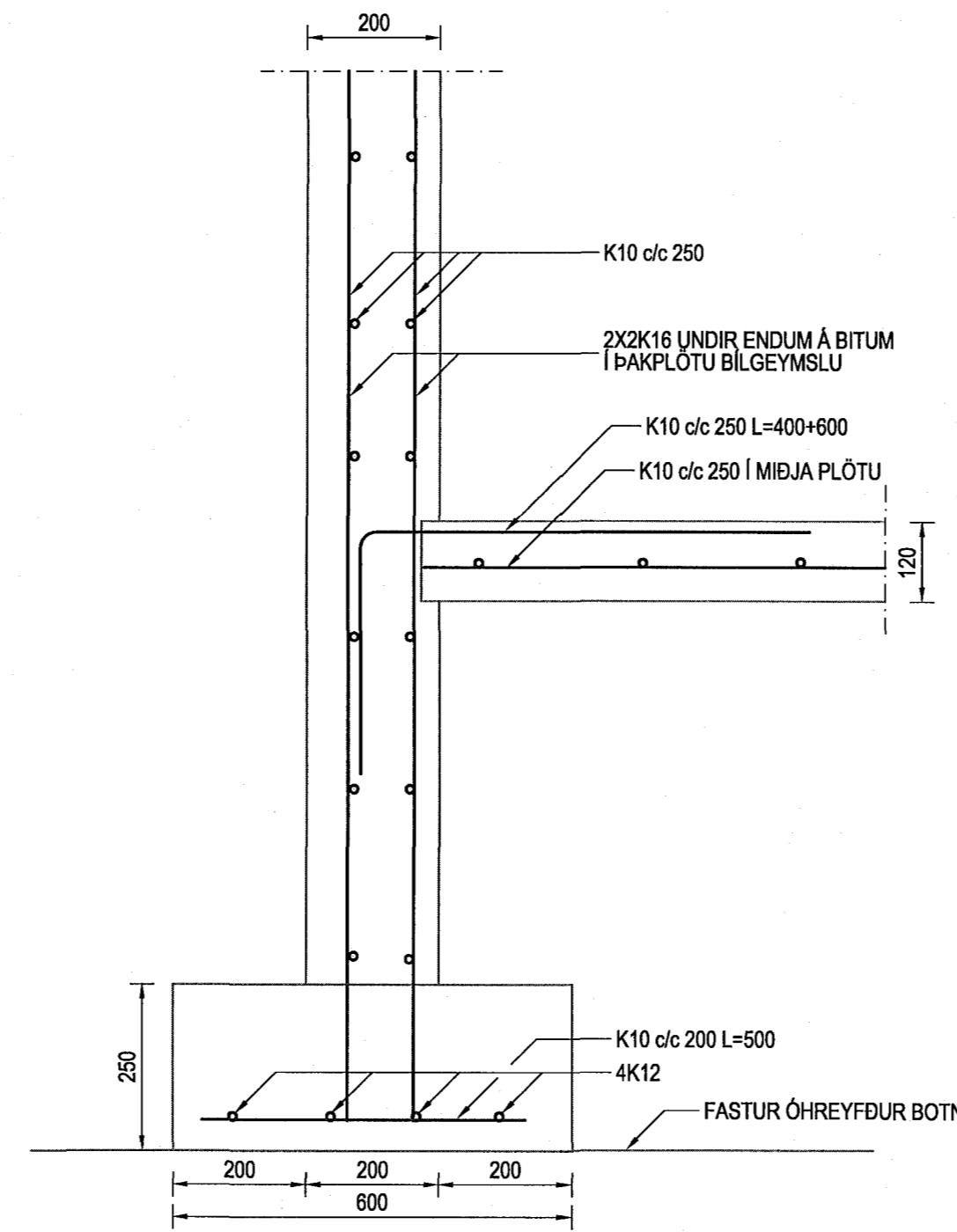
SNID 3-3 MKV. 1:10
