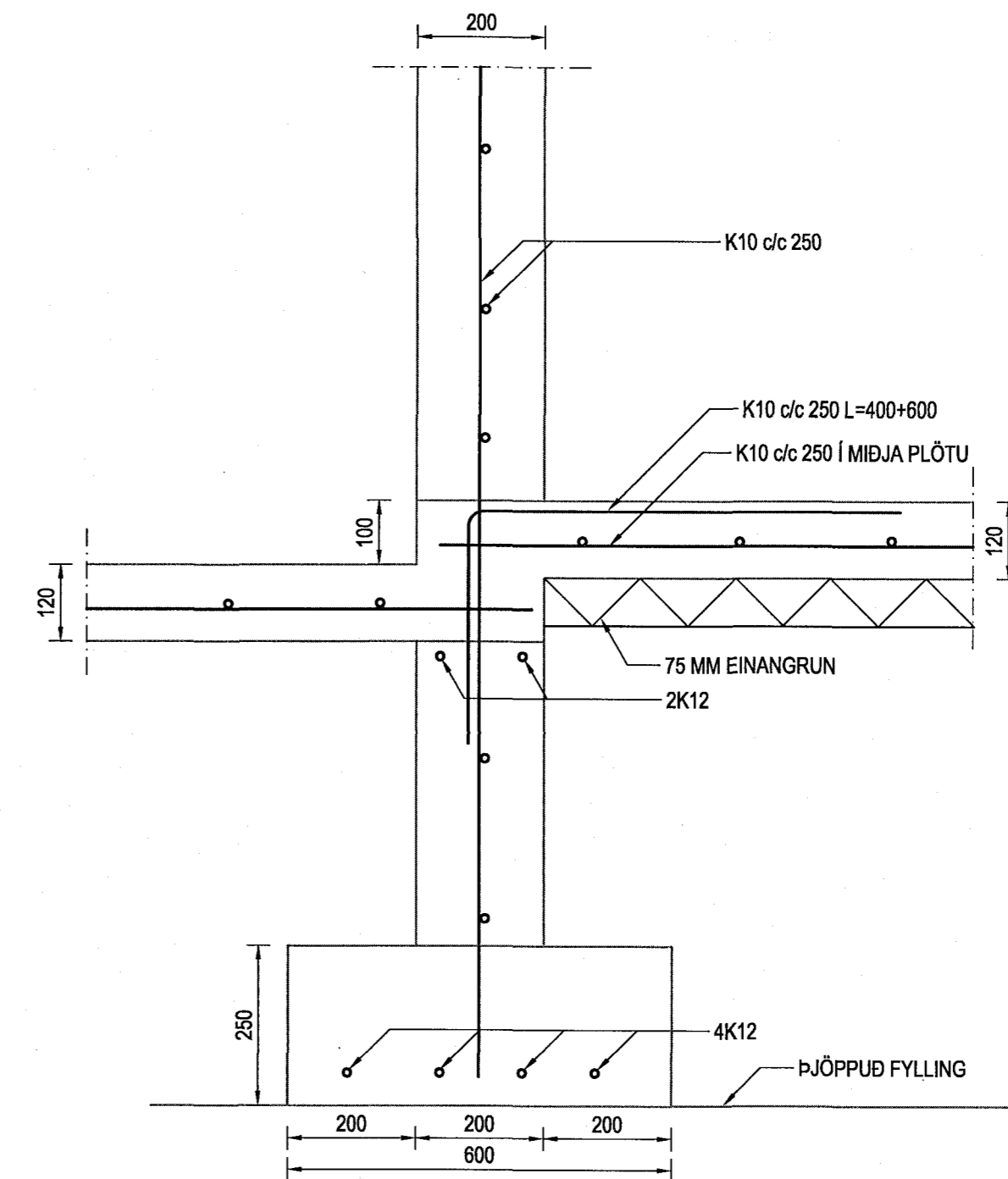
SNID 8-8 MKV. 1:10
