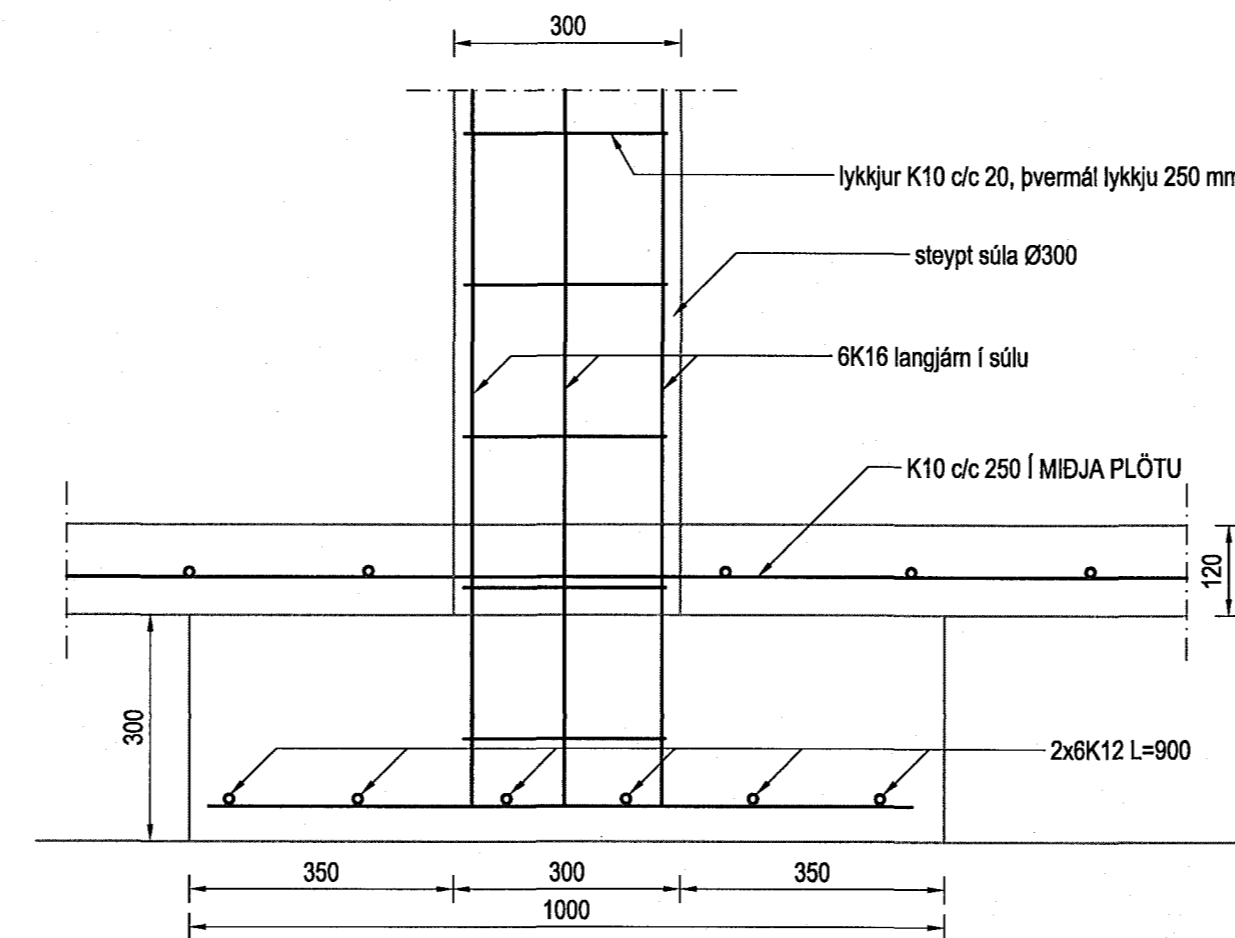
SNID 7-7 MKV. 1:10
