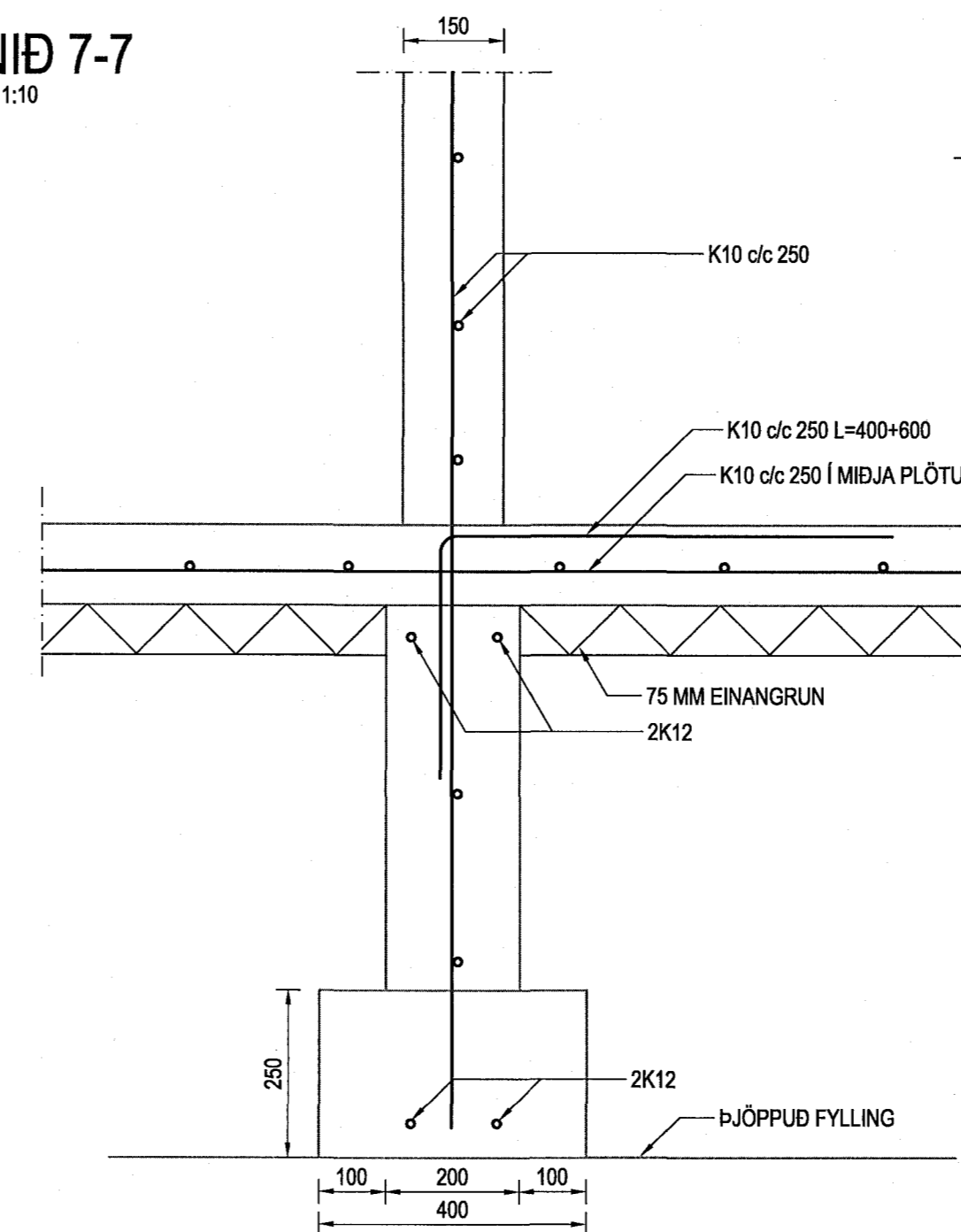
SNID 10-10 MKV. 1:10
